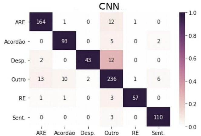
Figure 6 Confusion Matrix.
